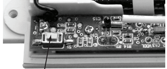
Connection button located inside the R250W
